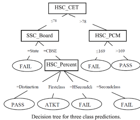
Fig 4: Decision tree
