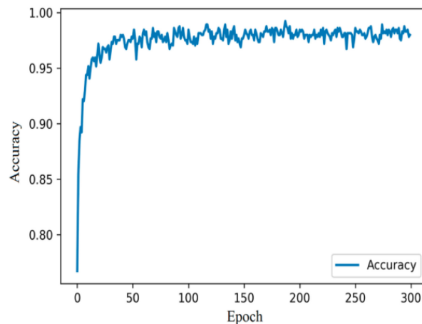
Fig:5 –Accuracy
